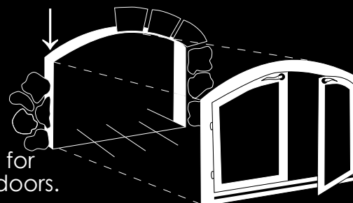
Mason's Template
