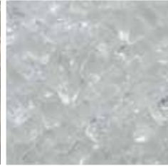
Starfire crystals
