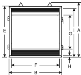
Louvered Fireboxes
