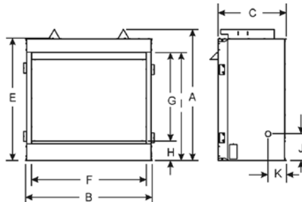
Flush Fireboxes
