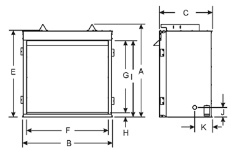
Select Fireboxes
